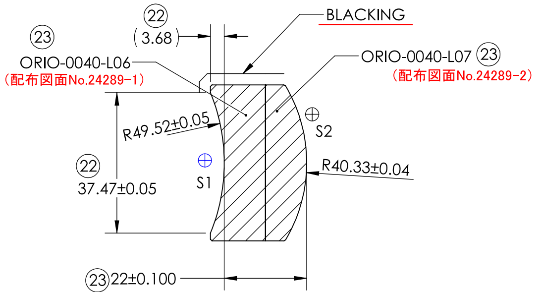
SECTION H-H SCALE 1 : 1
